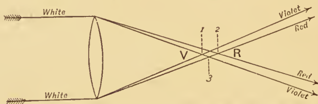
FIG. 65.—Showing the boundary rays of a parallel beam passing through a lens, and its violet and red foci.
